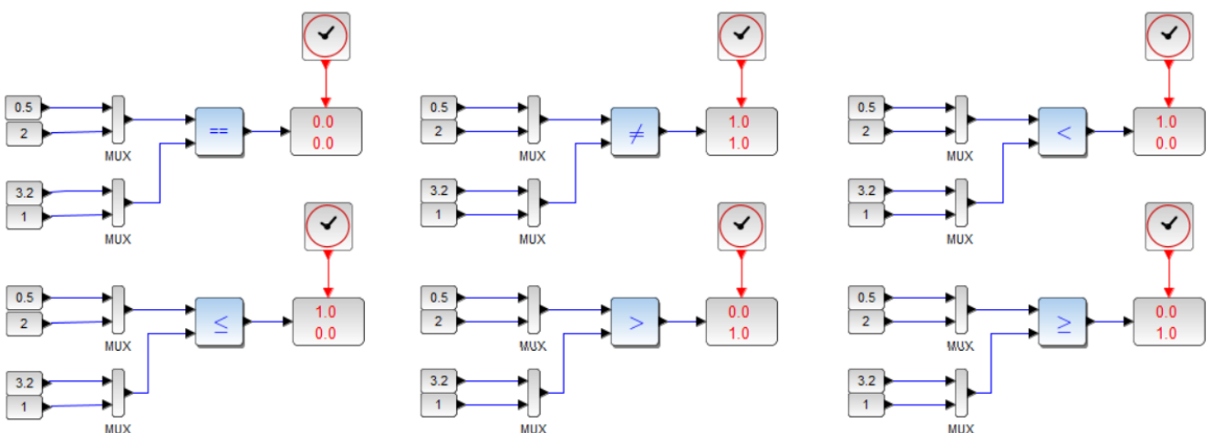
Figure 51 : Programme de test RELATION_OP multivariables.zcos
